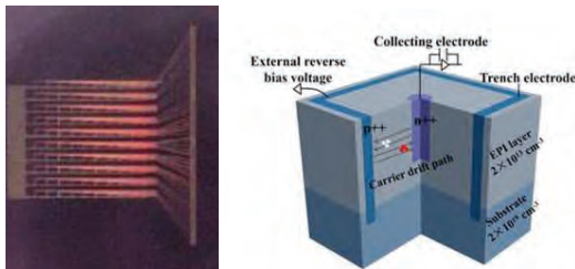
Figure 1. Microscopic image of Multi – array of 3D cylindrical IMECAS microdetectors b) 35 \times 35\ \mu\text{m}^2 IMECAS 3D cell with 0.5\ \mu\text{m} n+ central 3D electrode and p+ trench electrode in square shape.
