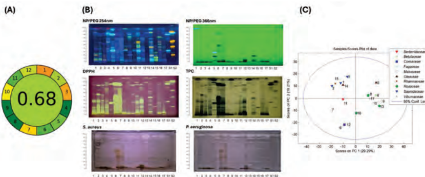
Figure 1. The integrated analytical workflow for seed extracts evaluation: (A) greenness assessment using AGREE; (B) HPTLC-based chemical and biological profiling; (C) principal component analysis.
