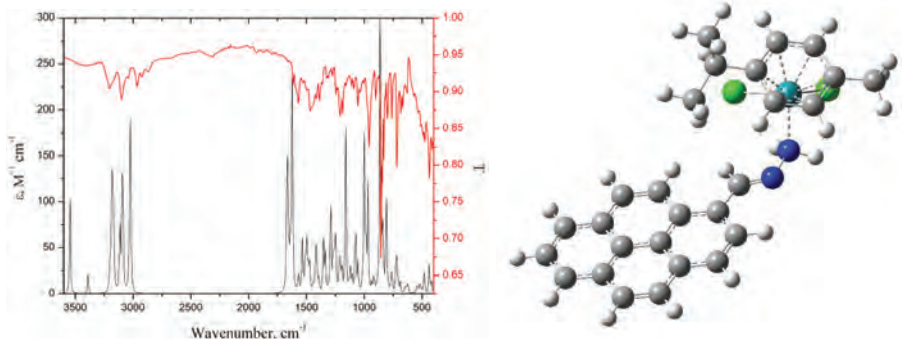
Figure 1. Experimental (red line) and theoretical (black line) FTIR spectra of [\text{RuCl}_2(\eta^6\text{-}p\text{-cymene})(1\text{-pcah-}\kappa\text{N})] (left); Optimized structure of the complex at the B3LYP/6-311++G(d,p)(H,C,N,Cl)/LanL2DZ(Ru) level of theory (right)
